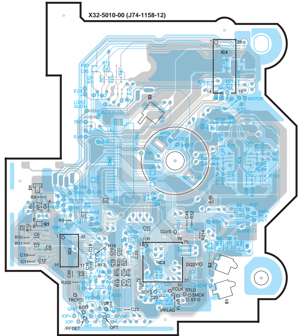
CD PLAYER UNIT (X32-5010-00)
